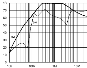
10 A type
