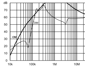
16 A type
